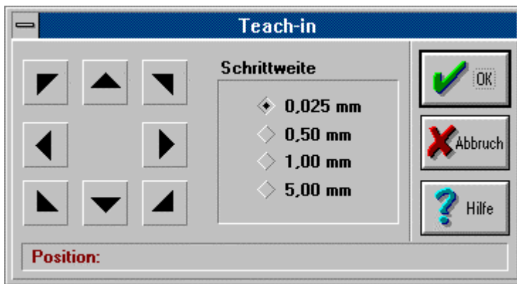
Abb 10 : Teach-In Dialog
